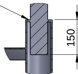
DETAIL AX SCALE 1 : 10
